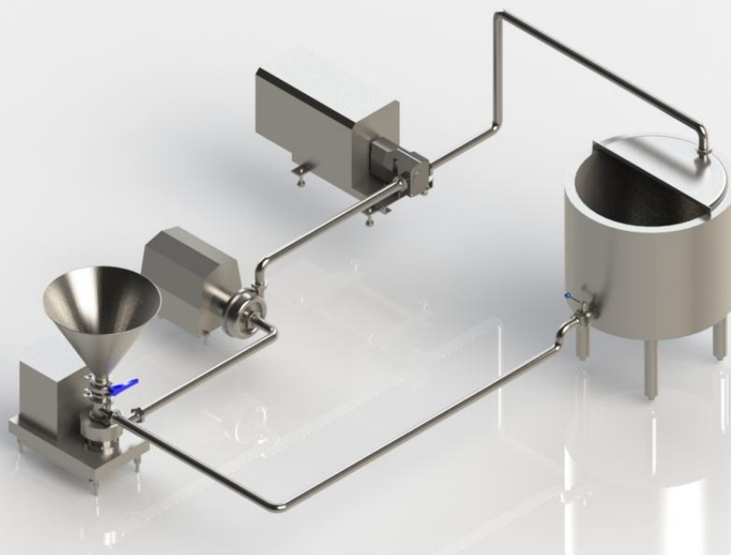
ILLUSTRATION ONLY FOR GENERAL PROCESS
